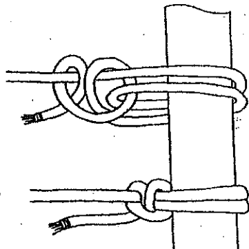
Fisherman's Hitch
