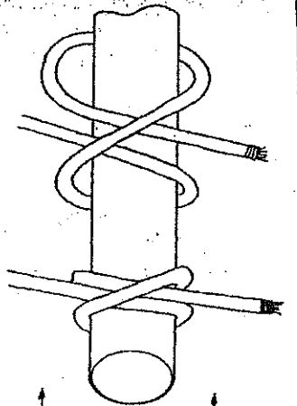
(led around a pipe) Clove Hitch
