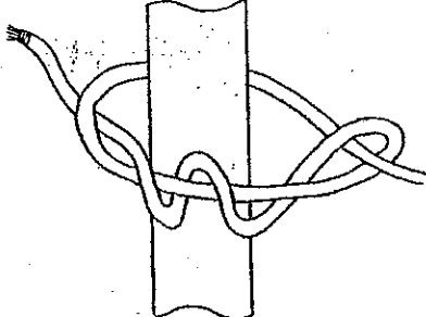
Timber Hitch
